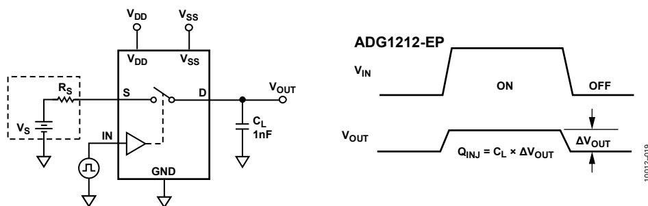
Figure 19. Charge Injection
