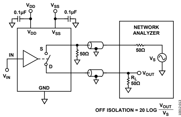
Figure 13. Off Isolation
