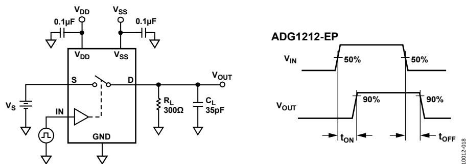
Figure 18. Switching Times
