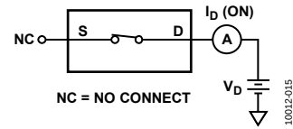
Figure 15. On Resistance
