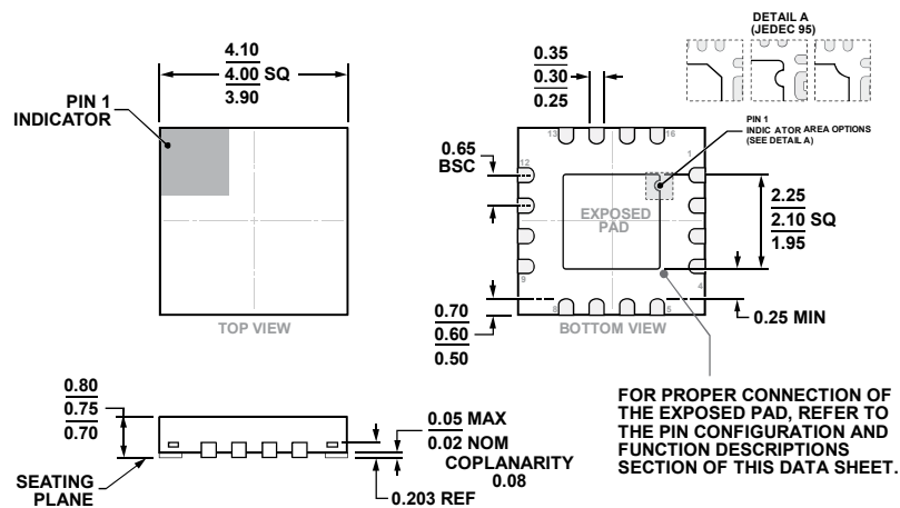
Figure 43. 16-Lead Lead Frame Chip Scale Package [LFCSP] 4 mm x 4 mm Body and 0.75 mm Package Height (CP-16-23)
