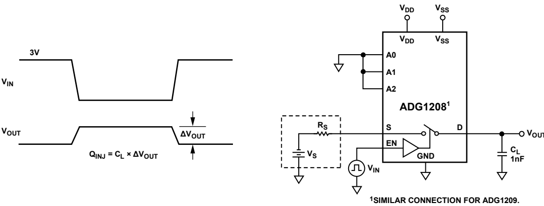
Figure 37. Charge Injection
