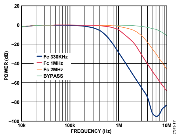
Figure 11. Rx Filter Performance, Power vs. Input Frequency
