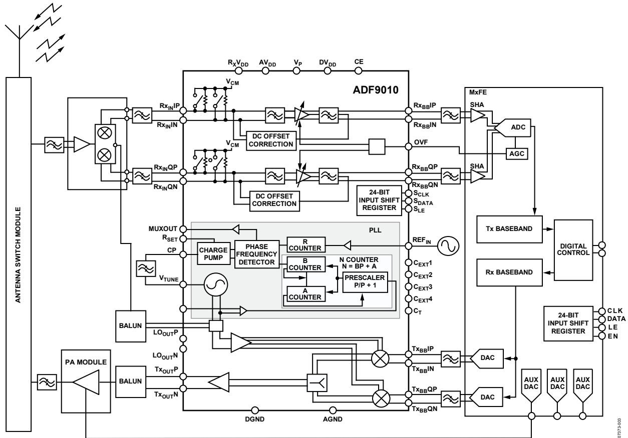
Figure 27. Applications Diagram
