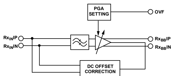
Figure 12. Rx Filter
