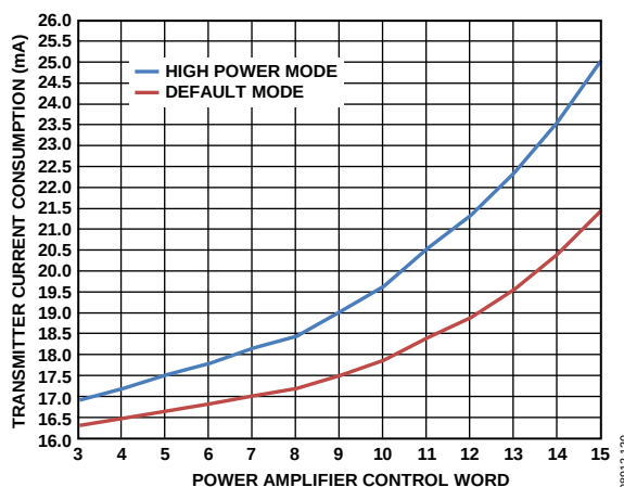
Figure 67. Transmitter Current Consumption vs. Control Word, for Default and High Power Modes, f_{\text{CHANNEL}} = 2.45 \text{ GHz} , V_{\text{DD\_BAT}} = 3.6 \text{ V} , Temperature = 25^\circ\text{C}
