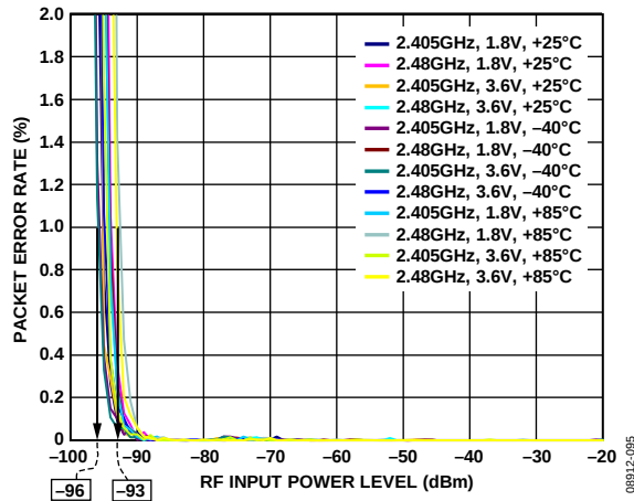
Figure 15. IEEE 802.15.4-2006 Packet Mode Sensitivity vs. Temperature and V_{DD\_BAT} , f_{CHANNEL} = 2.405\text{ GHz} , 2.45\text{ GHz} , 2.48\text{ GHz} , RFIO2
