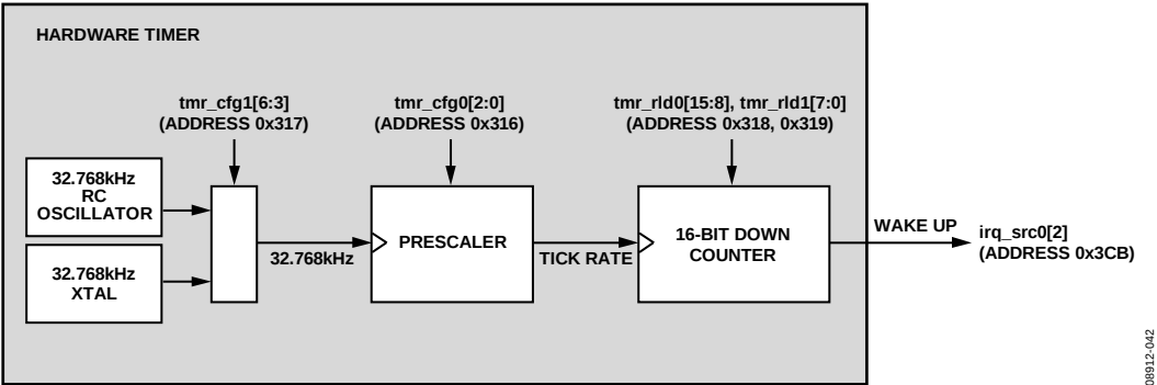
Figure 100. Hardware Wake-Up Timer Diagram
