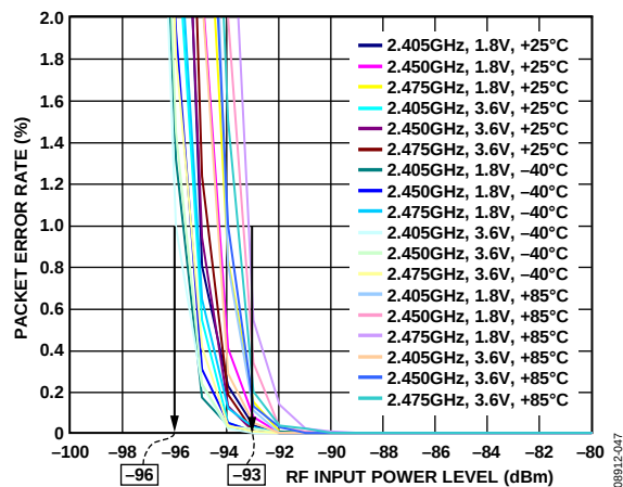
Figure 17. IEEE 802.15.4 Packet Mode Sensitivity vs. Temperature and V_{DD\_BAT} , f_{CHANNEL} = 2.405\text{ GHz} , 2.45\text{ GHz} , 2.475\text{ GHz} , RFIO1
