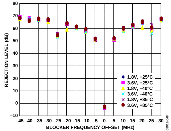
Figure 18. IEEE 802.15.4-2006 Packet Mode Blocker Rejection vs. Temperature and V_{DD\_BAT} , Modulated Blocker, P_{WANTED} = -85\text{ dBm} + 3\text{ dB} , f_{CHANNEL} = 2.45\text{ GHz} , RFIO2
