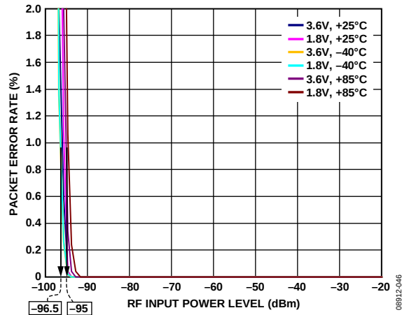
Figure 16. IEEE 802.15.4-2006 Packet Mode PER vs. RF Input Power Level vs. Temperature and V_{DD\_BAT} , f_{CHANNEL} = 2.45\text{ GHz} , RFIO2
