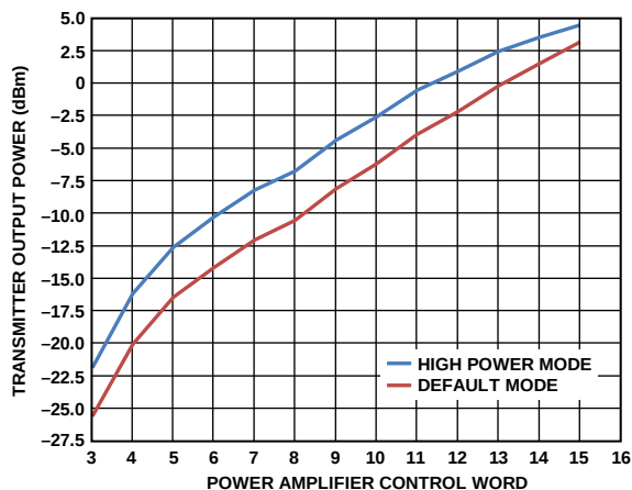
Figure 66. Transmitter Output Power vs. Control Word for Default and High Power Modes, f_{\text{CHANNEL}} = 2.45 \text{ GHz} , V_{\text{DD\_BAT}} = 3.6 \text{ V} , Temperature = 25^\circ\text{C} , RF Carrier Frequency, Temperature, and V_{\text{DD\_BAT}} (A discrete matching network and a harmonic filter are used as per the ADF7242 reference design.)
