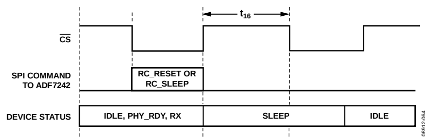
Figure 5. Wake-Up After an \text{RC\_RESET} or \text{RC\_SLEEP} Command
