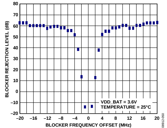
Figure 20. IEEE 802.15.4 Packet Mode Narrow-Band Blocker Rejection, CW Blocker, P_{WANTED} = -95\text{ dBm} + 3\text{ dB} , f_{CHANNEL} = 2.45\text{ GHz} , RFIO2
