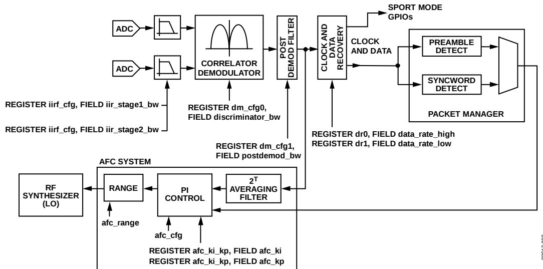
Figure 93. Structure of RX Demodulator
