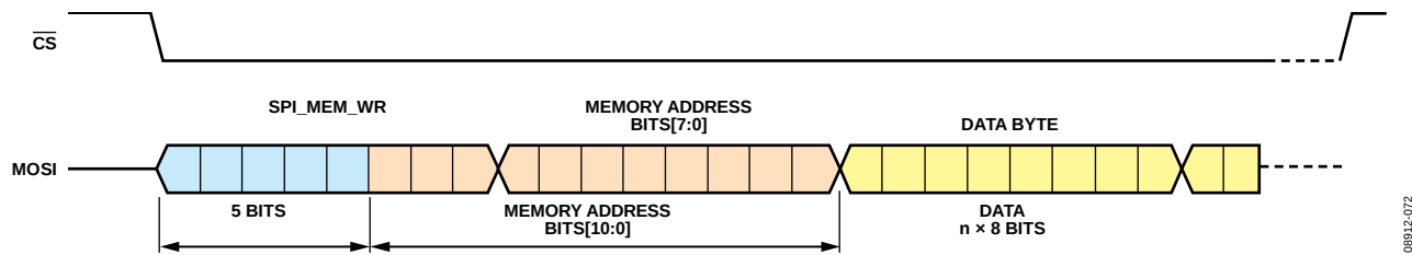
Figure 105. SPI Memory Access Command/Address Format
