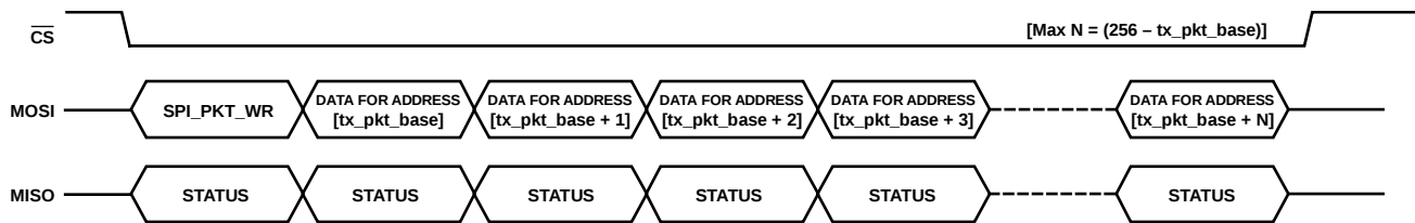
Figure 106. Packet RAM Write (tx_pkt_base is the address base pointer value for TX, which is programmed in Register txbp, Bit tx_pkt_base.)
