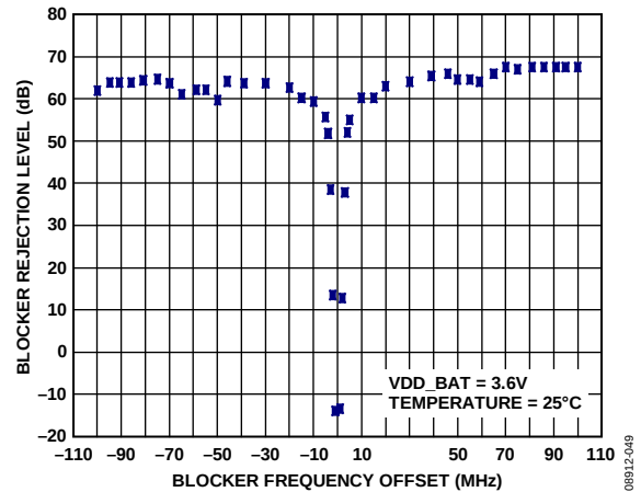
Figure 19. IEEE 802.15.4-2006 Packet Mode Wide-Band Blocker Rejection, CW Blocker, P_{WANTED} = -95\text{ dBm} + 3\text{ dB} , f_{CHANNEL} = 2.45\text{ GHz} , RFIO2
