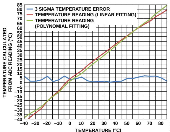
Figure 68. Temperature Sensor Performance (Average of 1000 ADC Readbacks) and 3\text{-}\Sigma Error vs. Temperature, V_{\text{DD\_BAT}} = 3.6 \text{ V}
