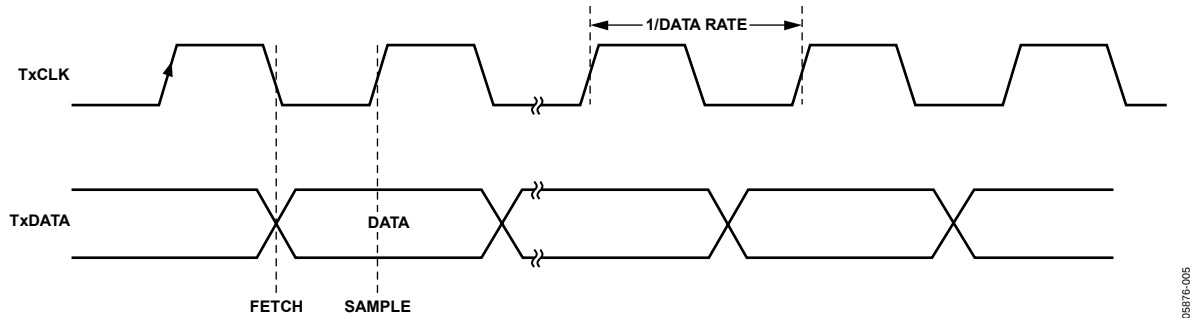
Figure 5. TxData/TxCLK Timing Diagram
