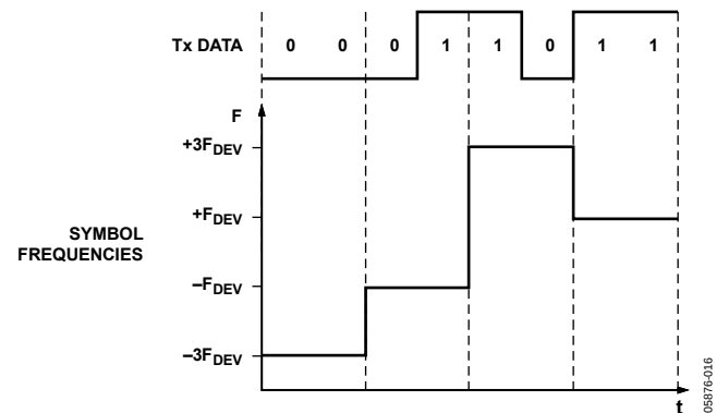
Figure 18. 4FSK Encoding
