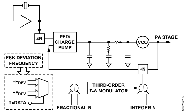
Figure 16. 2FSK Implementation
