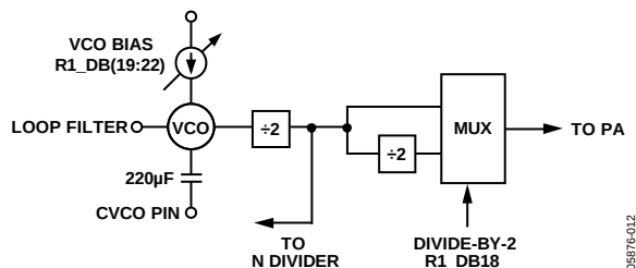
Figure 36. Voltage Controlled Oscillator (VCO)
