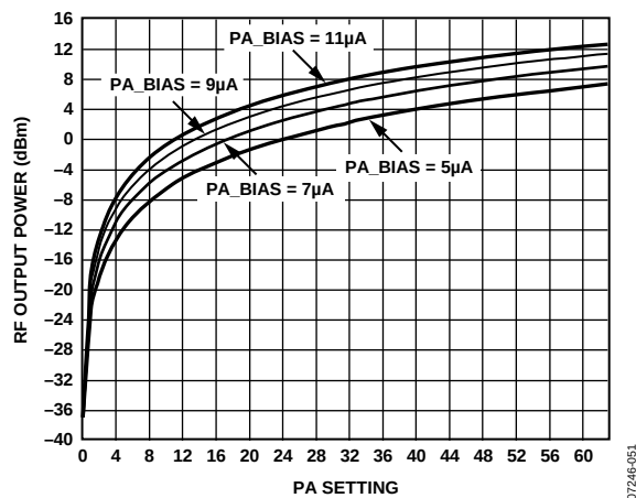
Figure 12. RF Output Power vs. PA Setting
