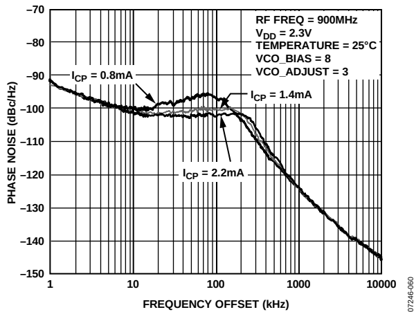
Figure 11. Phase Noise Response at 900 MHz, V_{DD} = 2.3\text{ V}
