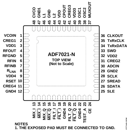
Figure 10. Pin Configuration
