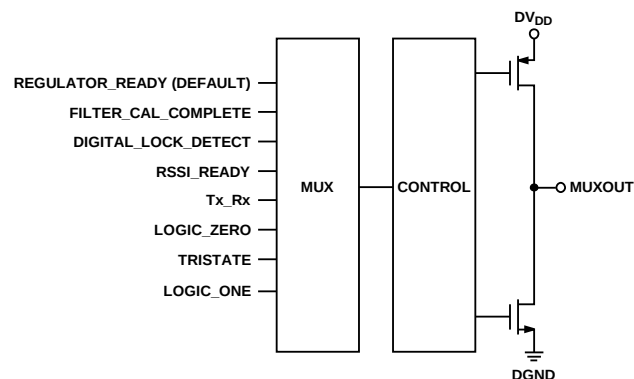
Figure 36. MUXOUT Circuit
