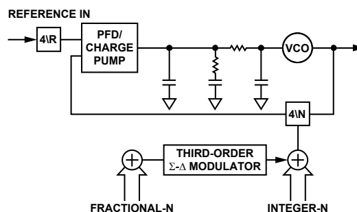
Figure 23. Fractional-N PLL
