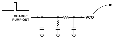
Figure 22. Typical Loop-Filter Configuration
