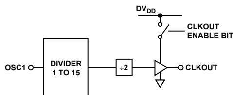
Figure 20. CLKOUT Stage
