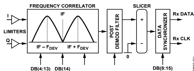
Figure 31. FSK Correlator/Demodulator Block Diagram
