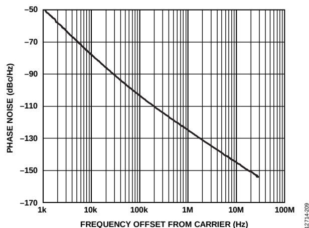
Figure 9. Open-Loop VCO Phase Noise, 13.6 GHz
