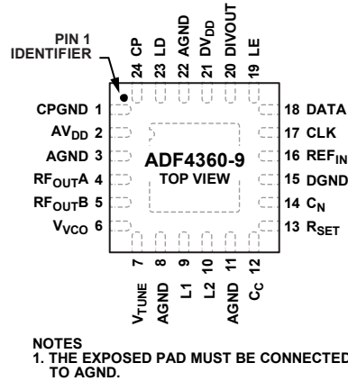
Figure 3. Pin Configuration
