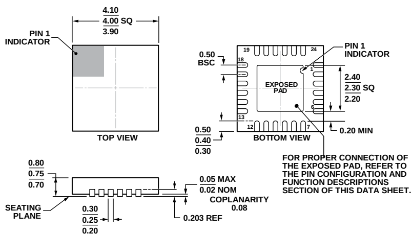
Figure 36. 24-Lead Lead Frame Chip Scale Package [LFCS] 4 mm × 4 mm Body and 0.75 mm Package Height (CP-24-14) Dimensions shown in millimeters
