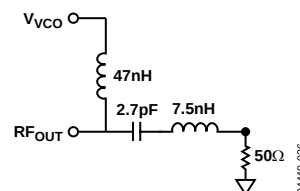
Figure 22. Optimum ADF4360-6 Output Stage
