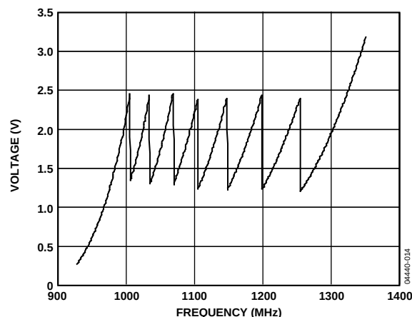
Figure 14. Frequency vs. V_{TUNE} , ADF4360-6
