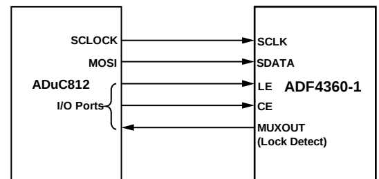
Figure 19. ADuC812 to ADF4360-1 Interface
