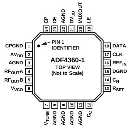
Figure 3. Pin Configuration
