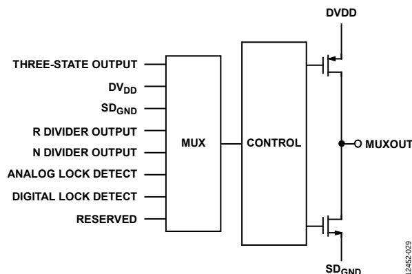
Figure 25. MUXOUT Schematic
