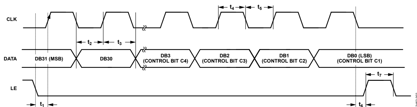
Figure 2. Timing Diagram
