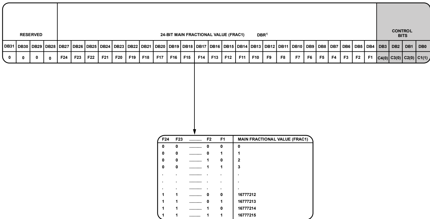
Figure 31. Register 1
