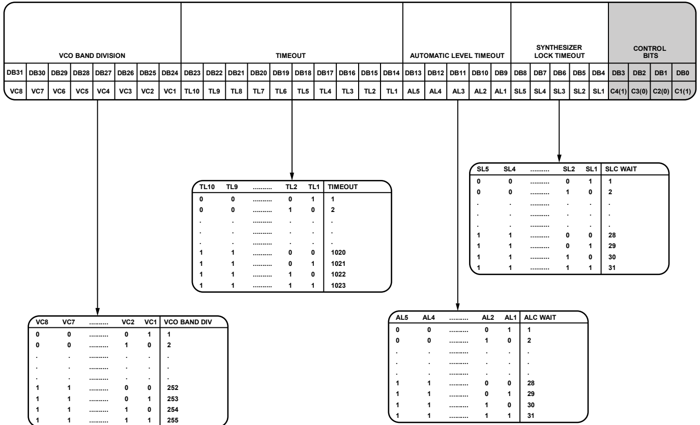
Figure 39. Register 9
