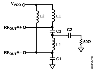
Figure 39. LC Balun for the ADF4351
