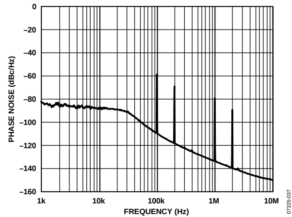
Figure 13. Fractional-N Spur Performance. Low Noise Mode, R_{FOUT} = 2.591 GHz, R_{FIN} = 105 MHz, PFD = 17.5 MHz, Output Divide-by-1 Selected; Loop Filter Bandwidth = 20 kHz, Channel Spacing = 100 kHz.
