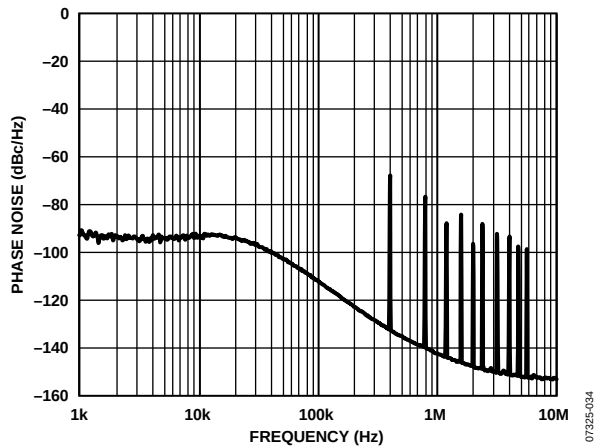
Figure 10. Integer-N Phase Noise and Spur Performance. GSM900 Band, R_{FOUT} = 904 MHz, R_{FIN} = 100 MHz, PFD = 800 kHz, Output Divide-by-4 Selected; Loop-Filter Bandwidth = 16 kHz, Channel Spacing = 200 kHz.
