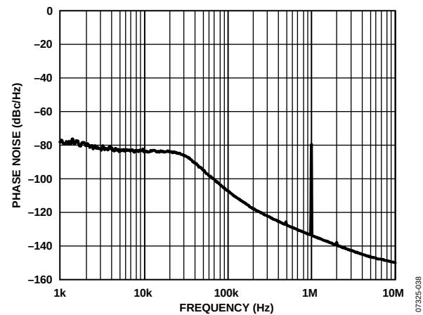
Figure 14. Fractional-N Spur Performance. Low Spur Mode R_{FOUT} = 2.591 GHz, R_{FIN} = 105 MHz, PFD = 17.5 MHz, Output Divide-by-1 Selected. Loop Filter Bandwidth = 20 kHz, Channel Spacing = 100 kHz (Note That Fractional Spurs Are Removed and Only the Integer Boundary Spur Remains in Low Spur Mode).
