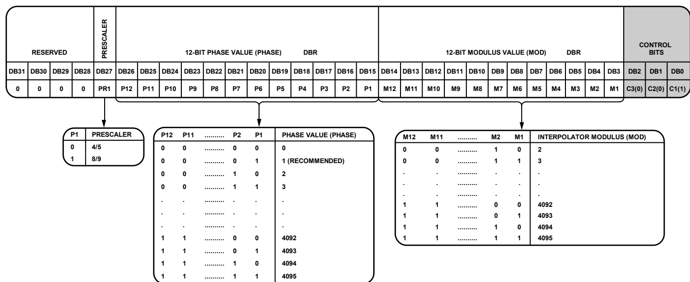
Figure 25. Register 1 (R1)
