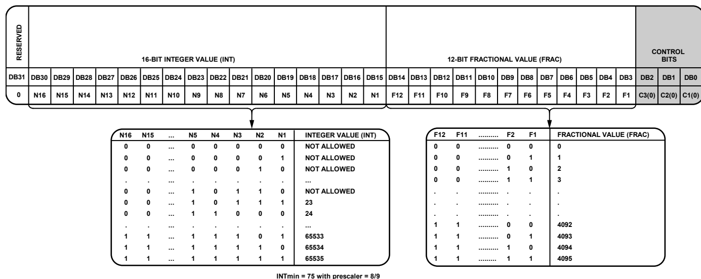
Figure 24. Register 0 (R0)
