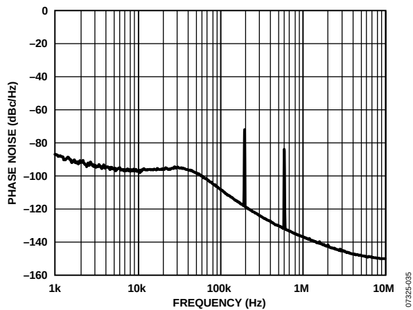
Figure 11. Fractional-N Spur Performance; Low Noise Mode. W-CDMA Band, R_{FOUT} = 2113.5 MHz, R_{FIN} = 100 MHz, PFD = 25 MHz, Output Divide-by-2 Selected; Loop Filter Bandwidth = 40 kHz, Channel Spacing = 200 kHz.
