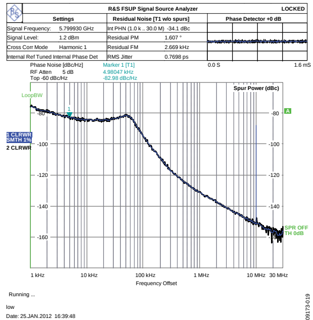
Figure 19. Spectrum Analyzer Display
