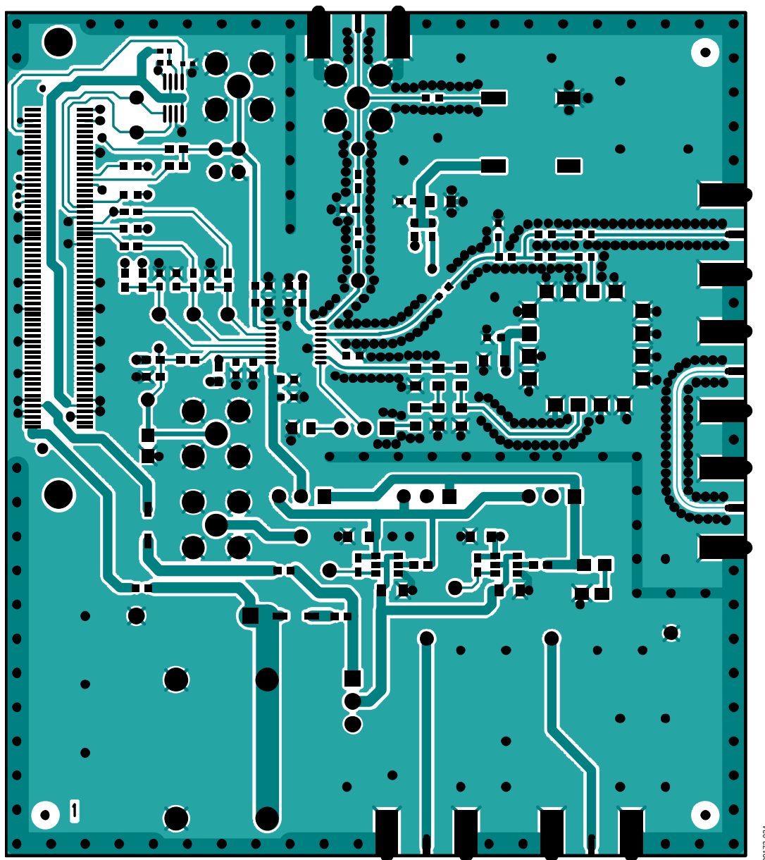
Figure 24. Top Side
