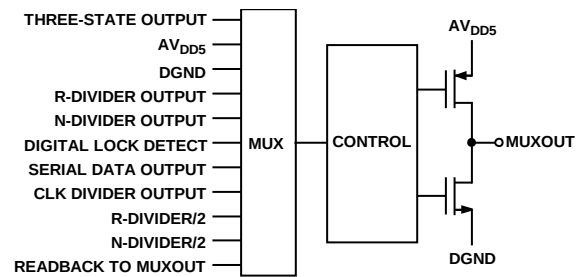
Figure 19. MUXOUT Schematic
