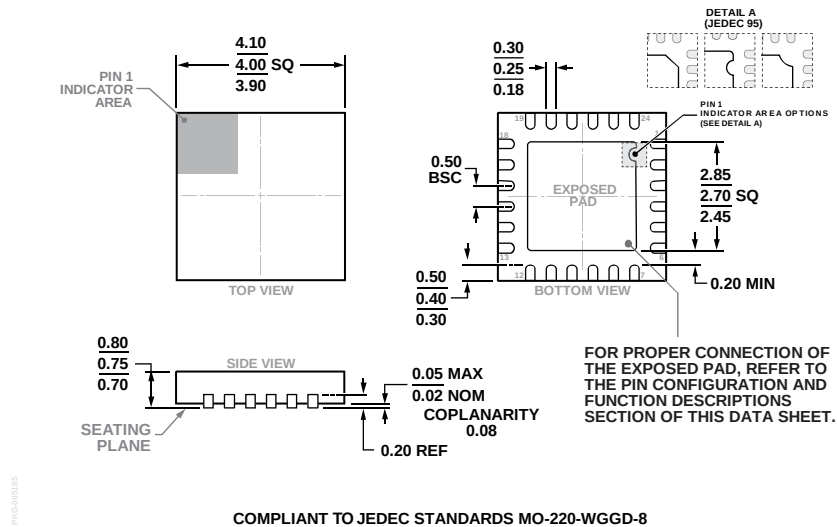
Figure 38. 24-Lead Lead Frame Chip Scale Package [LFCSP] 4 mm × 4 mm Body and 0.75 mm Package Height (CP-24-8)
