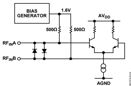
Figure 15. RF Input Stage
