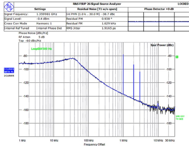
Figure 19. Signal Source Analyzer Display
