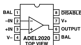
8-Lead PDIP (N)
