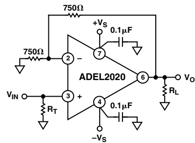
Figure 7. Connection Diagram for A_{VCL} = +2
