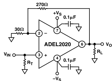
Figure 8. Connection Diagram for A_{VCL} = +10
