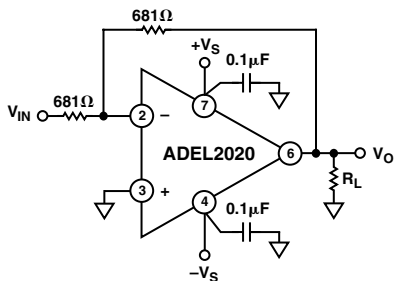
Figure 6. Connection Diagram for A_{VCL} = -1
