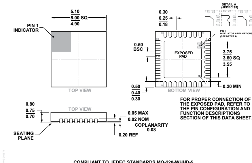
Figure 61. 32-Lead Lead Frame Chip Scale Package [LFCSP] 5 mm × 5 mm Body and 0.75 mm Package Height (CP-32-12) Dimensions shown in millimeters
