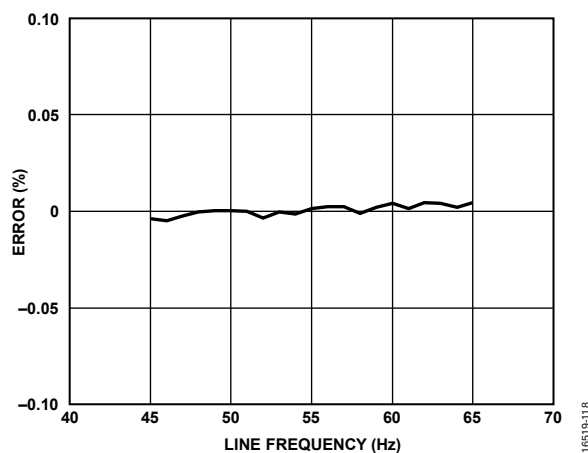
Figure 18. Total Apparent Energy Error vs. Line Frequency, AI PGA Gain = 38.4x
