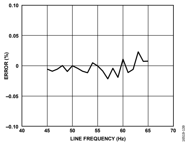
Figure 32. Voltage Channel RMS Overcurrent Error vs. Line Frequency
