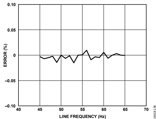
Figure 31. Current Channel B RMS Overcurrent Error vs. Line Frequency
