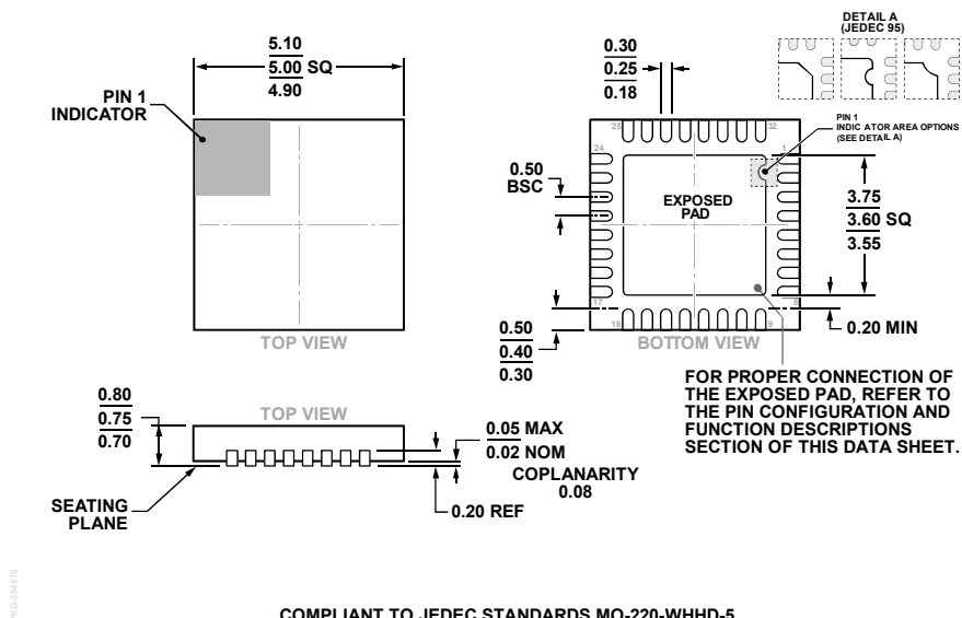
Figure 61. 32-Lead Lead Frame Chip Scale Package [LFCSP] 5 mm × 5 mm Body and 0.75 mm Package Height (CP-32-12)
