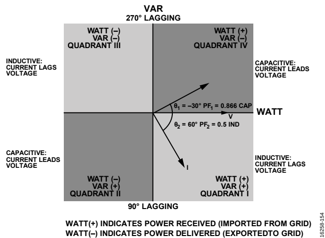
Figure 54. WATT and VAR Power Sign for Capacitive and Inductive Loads
