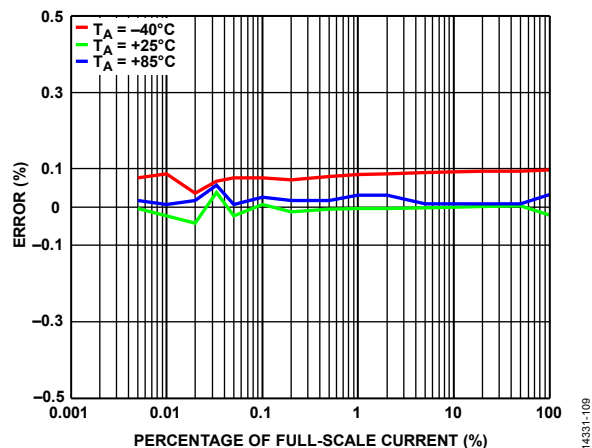
Figure 10. Fundamental Reactive Energy Error as a Percentage of Reading over Temperature, PF = 0
