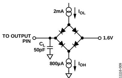
Figure 9. Load Circuit for Timing Specifications
