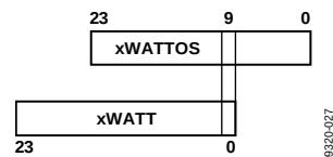
Figure 58. xWATTOS and xWATT Registers
