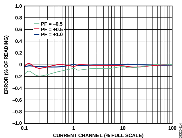
Figure 18. Current Channel B Active Energy Error as a Percentage of Reading (Gain = 1, Temperature = 25°C) over Power Factor with Internal Reference, Integrator Off
