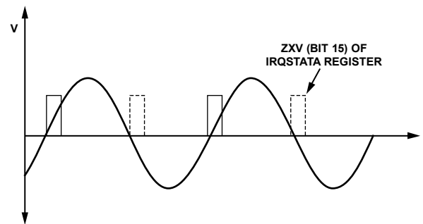
Figure 63. Zero-Crossing Interrupt
