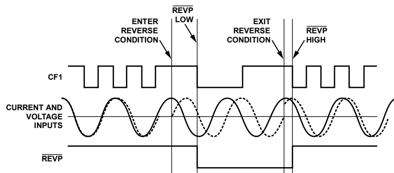
Figure 65. \overline{\text{REVP}} Output
