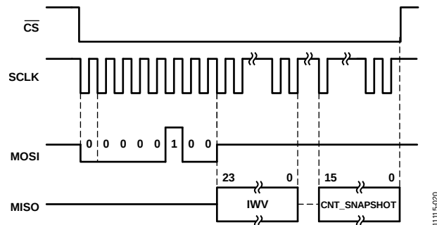
Figure 41. SPI Read Operation in Burst Mode
