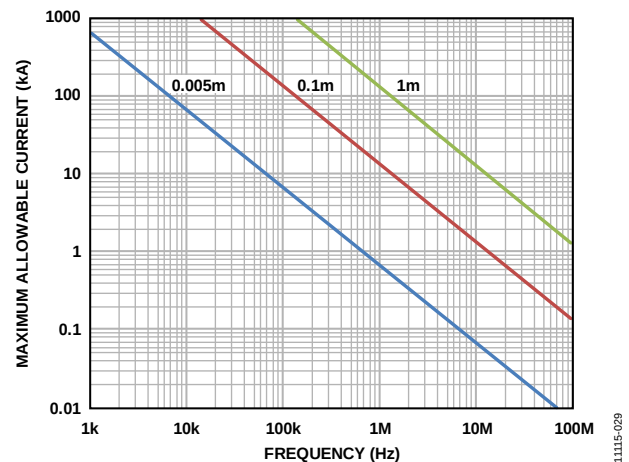
Figure 50. Maximum Allowable Current for Various Current-to-ADE7912/ADE7913 Spacings
