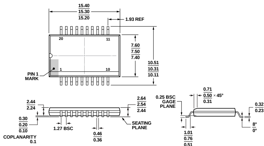
Figure 54. 20-Lead Standard Small Outline Package, with Increased Creepage [SOIC_IC] Wide Body (RI-20-1)
