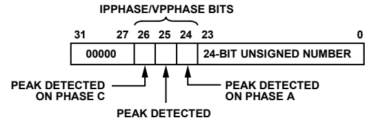
Figure 60. Composition of IPEAK[31:0] and VPEAK[31:0] Registers
