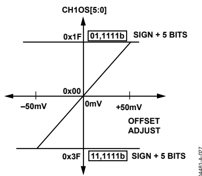
Figure 26. Channel 1 Offset Correction Range (Gain = 1)
