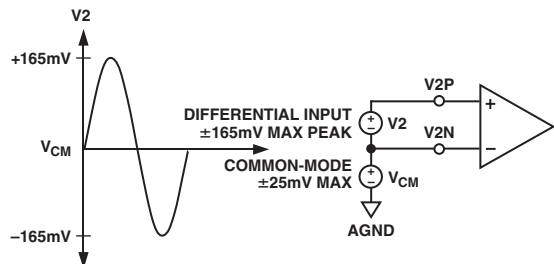
Figure 6. Maximum Signal Levels, Channel V2
