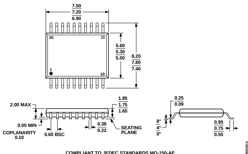
COMPLIANT TO JEDEC STANDARDS MO-150-AE Figure 98. 20-Lead Shrink Small Outline Package [SSOP] (RS-20)
