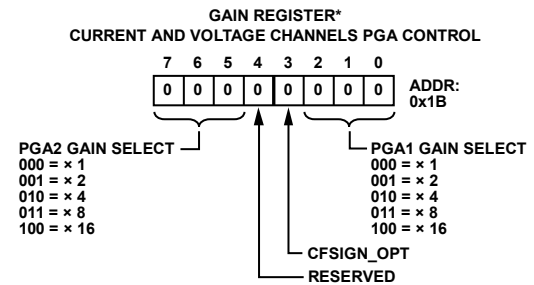
Figure 41. Analog Gain Register
