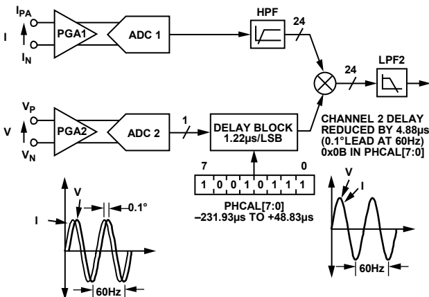
Figure 59. Phase Calibration
