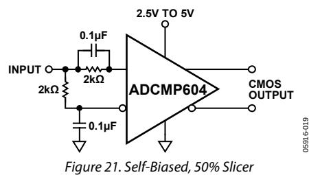
Figure 21. Self-Biased, 50% Slicer
