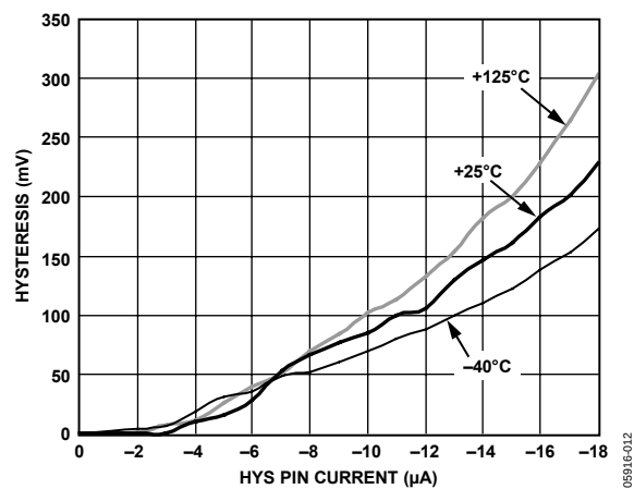
Figure 11. Hysteresis vs. Pin Current
