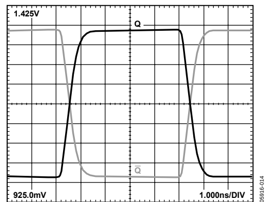
Figure 15. 50 MHz Output Voltage Waveform V_{CC} = 2.5\text{ V}
