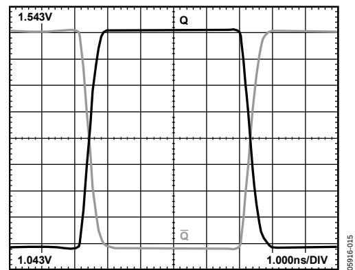
Figure 16. 50 MHz Output Voltage Waveform V_{CC} = 5.5\text{ V}
