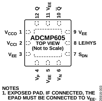
Figure 4. ADCMP605 Pin Configuration
