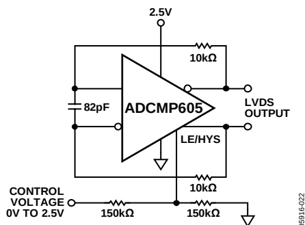
Figure 24. Voltage-Controlled Oscillator
