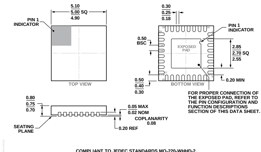
Figure 24. 32-Lead Lead Frame Chip Scale Package [LFCSP] 5 mm × 5 mm Body and 0.75 mm Package Height (CP-32-21) Dimensions shown in millimeters
