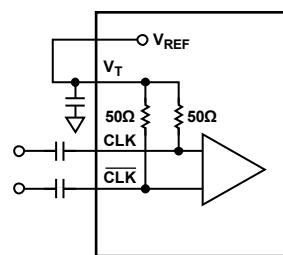
Figure 21. AC-Coupling Differential Signals Inputs, Such as LVDS
