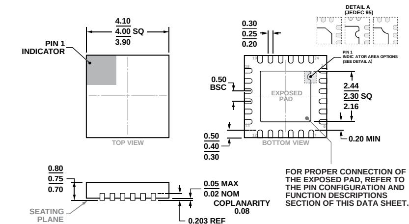
Figure 23. 24-Lead Lead Frame Chip Scale Package [LFCSP] 4 mm × 4 mm Body and 0.75 mm Package Height CP-24-14 Dimensions shown in millimeters
