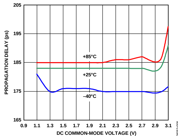
Figure 8. Propagation Delay vs. Common-Mode Voltage vs. Temperature, Input Slew Rate > 25\text{ V/ns}
