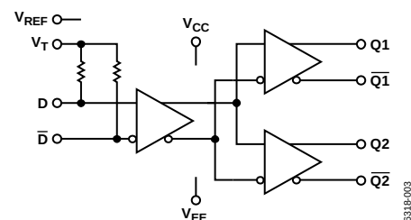
Figure 3. ADCLK925 ECL 1:2 Clock/Data Fanout Buffer
