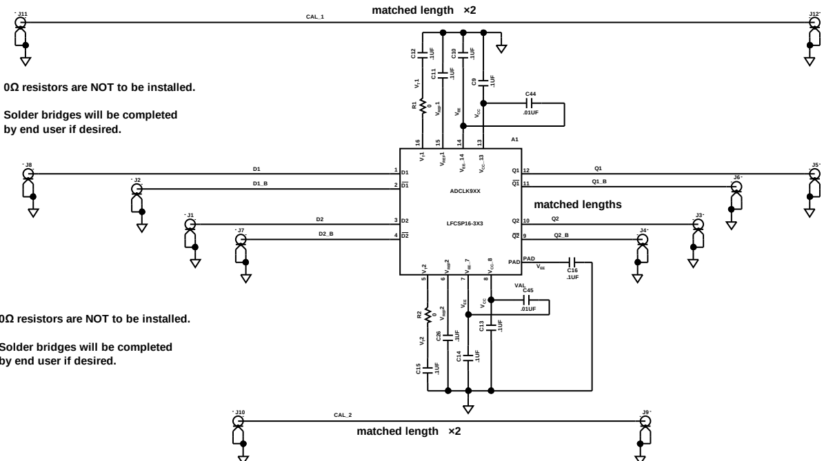
Figure 30. Evaluation Board Schematic
