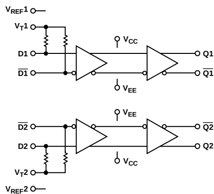
Figure 2. ADCLK907 ECL Dual 1:1 Clock/Data Buffer
