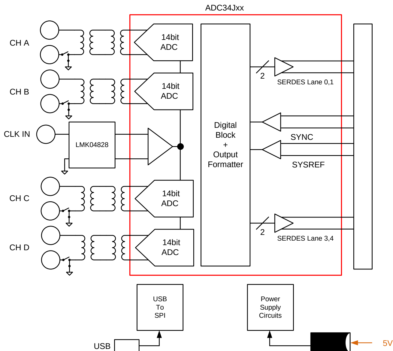
Figure 2. Simplified ADC34J4x EVM Block Diagram
