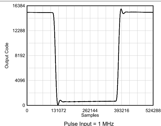
Figure 6-35. Pulse Response
