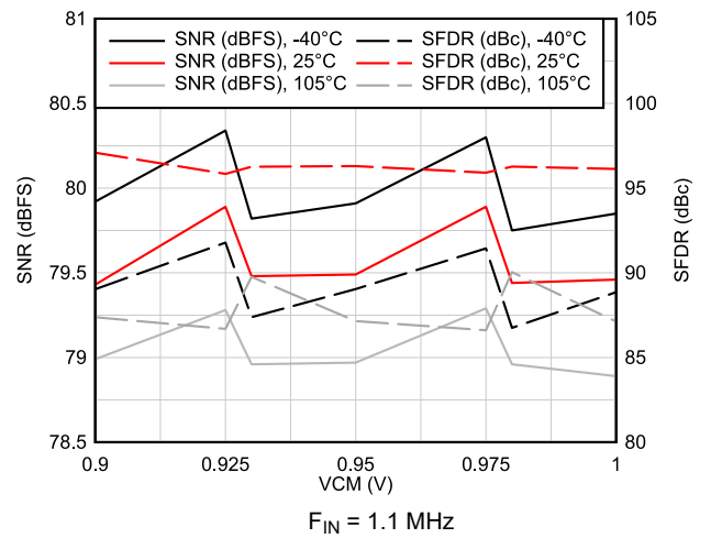
Figure 6-10. AC Performance vs VCM vs Temperature
