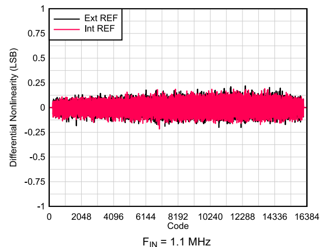
Figure 6-33. DNL vs Code
