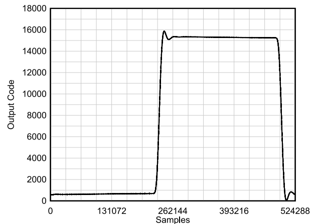
Figure 6-14. Pulse Response
