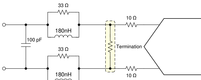
Figure 8-4. Sampling glitch filter example for input frequencies from DC to 30 MHz
