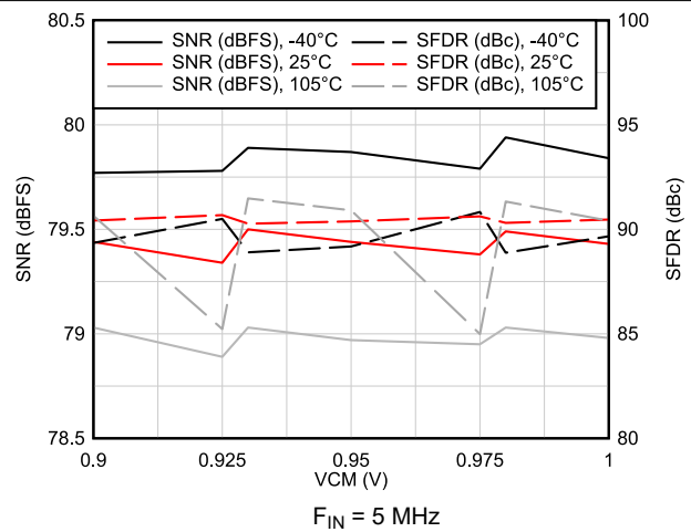
Figure 6-54. AC Performance vs VCM vs Temperature
