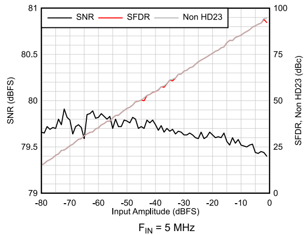
Figure 6-50. AC Performance vs Input Amplitude
