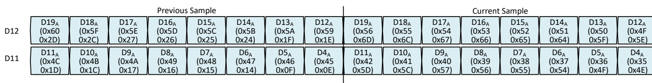
Figure 8-46. Example: 2-wire output mapping
