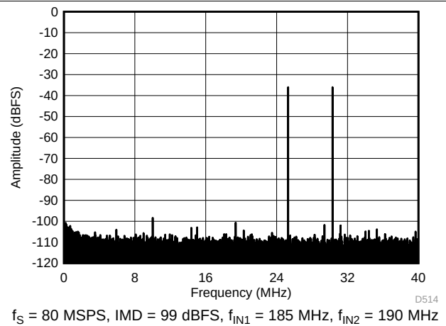
Figure 80. FFT for Two-Tone Input Signal ( -36\text{ dBFS} at 185\text{ MHz} and 190\text{ MHz} )
