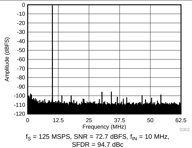
Figure 35. FFT for 10-MHz Input Signal (Dither Off)
