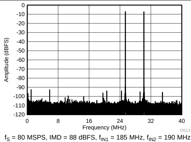
Figure 79. FFT for Two-Tone Input Signal ( -7\text{ dBFS} at 185\text{ MHz} and 190\text{ MHz} )
