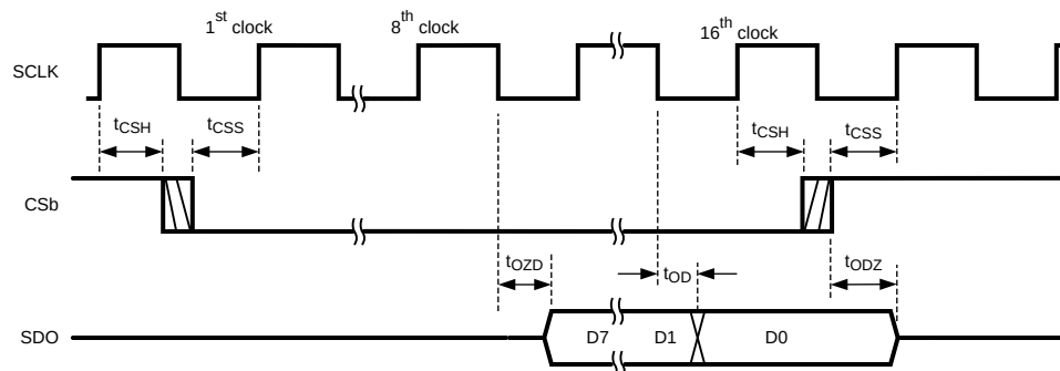
Figure 23. Read Timing
