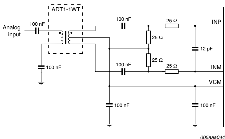
Fig 10. Single transformer configuration suitable for baseband applications
