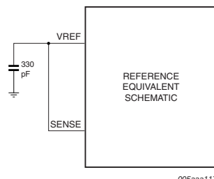
Fig 14. Internal reference, 1 V (p-p) full-scale
