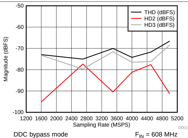
Figure 19. THD, HD2, HD3 vs Sampling Rate
