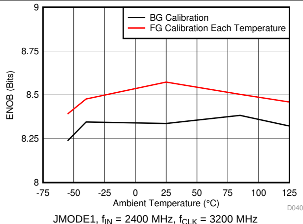
Figure 34. ENOB vs Temperature and Calibration Type
