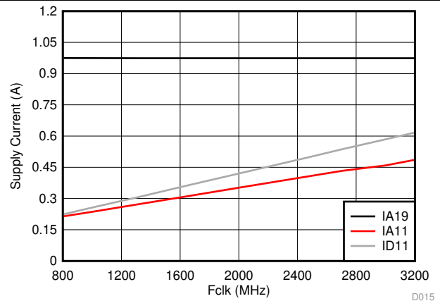
Figure 45. Supply Current vs Clock Frequency
