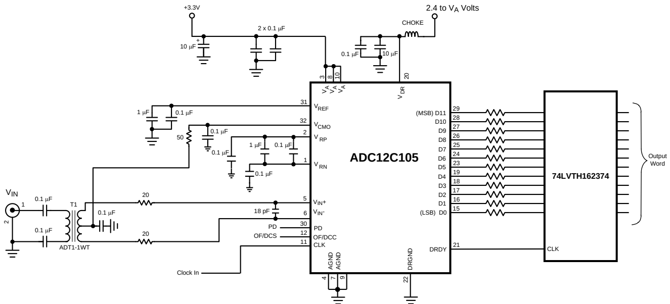
Figure 34. Application Circuit
