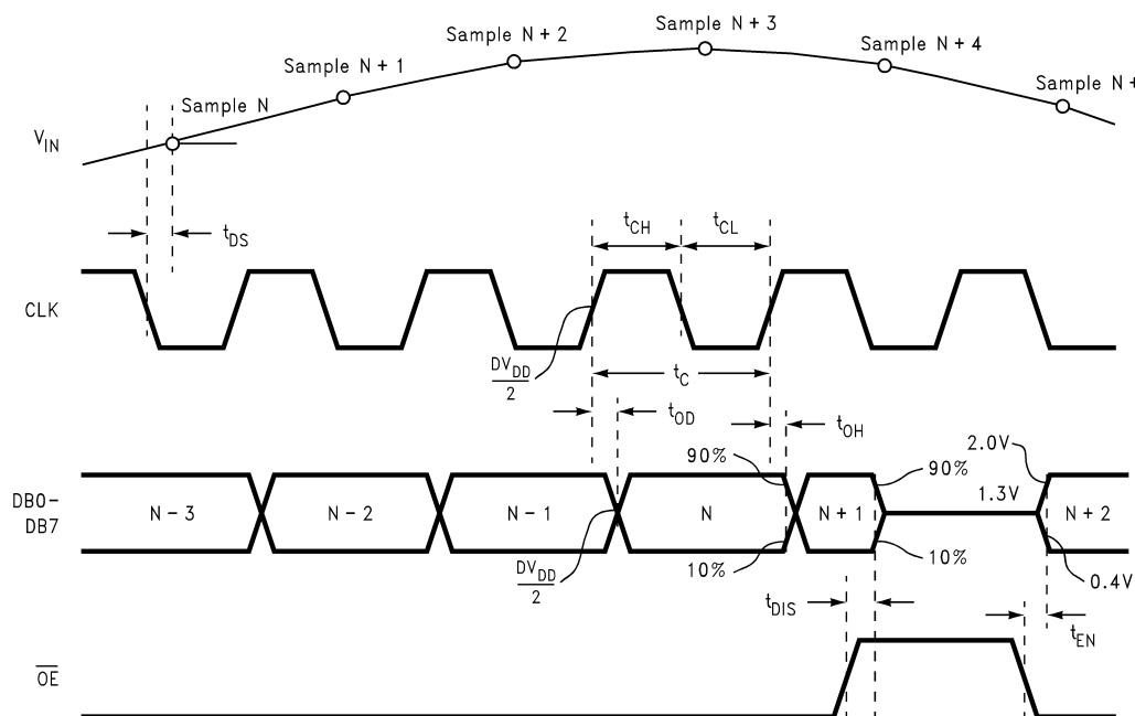
Figure 24. Timing Diagram
