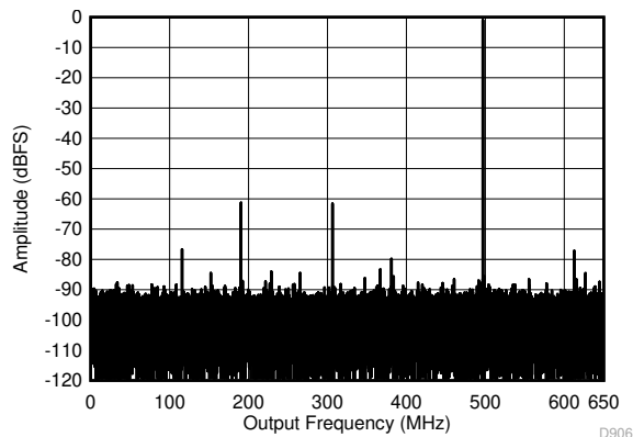
Figure 7-8. Single Tone FFT at 1797 MHz and -1 dBFS
