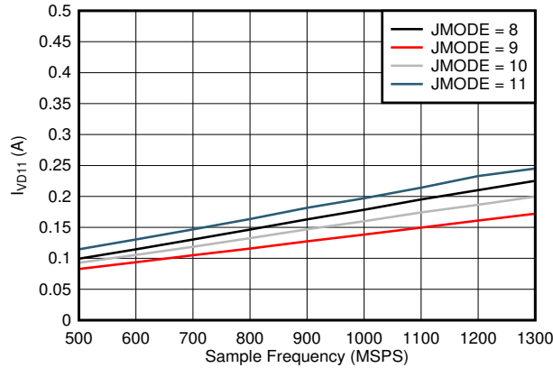
independent of power mode Figure 7-109. Single Channel, I_{VD11} vs FS and JMODE 8 - 11
