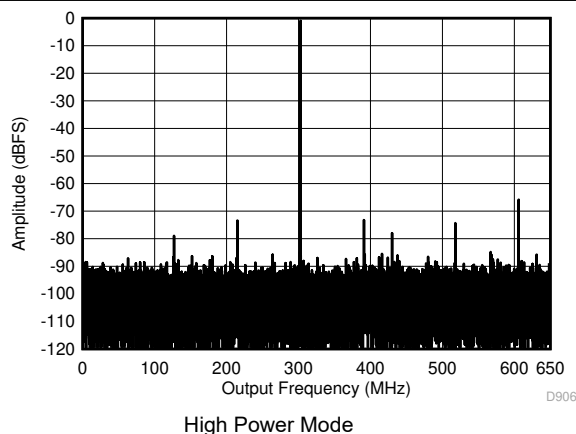
Figure 7-6. Single Tone FFT at 997 MHz and -1 dBFS
