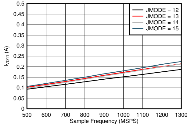
independent of power mode Figure 7-110. Single Channel, I_{VD11} vs FS and JMODE 12 - 15
