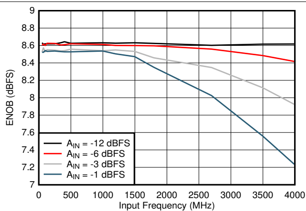
Figure 7-18. ENOB vs Input Frequency
