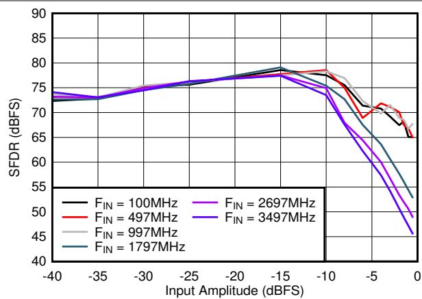
Figure 7-29. SFDR vs Input Amplitude
