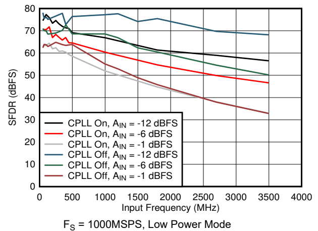
Figure 7-76. SFDR vs Input Frequency, CPLL and Input Amplitude
