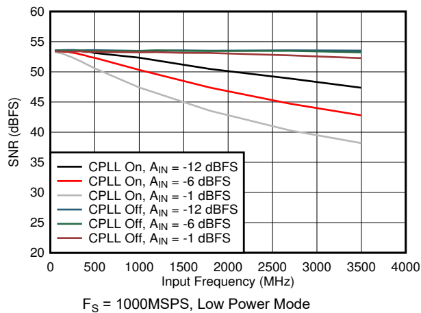
Figure 7-75. SNR vs Input Frequency, CPLL and Input Amplitude
