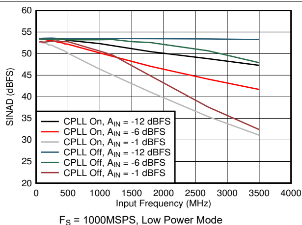
Figure 7-77. SINAD vs Input Frequency, CPLL and Input Amplitude
