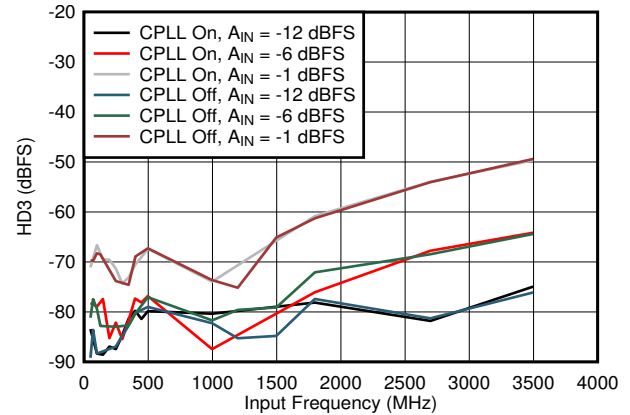
Figure 7-74. HD3 vs Input Frequency, CPLL and Input Amplitude
