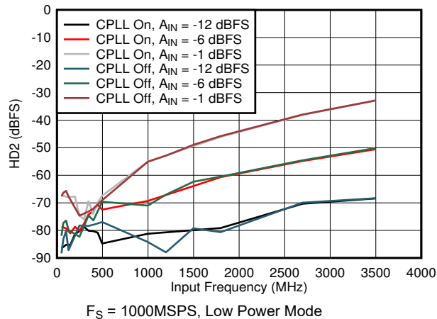
Figure 7-79. HD2 vs Input Frequency, CPLL and Input Amplitude
