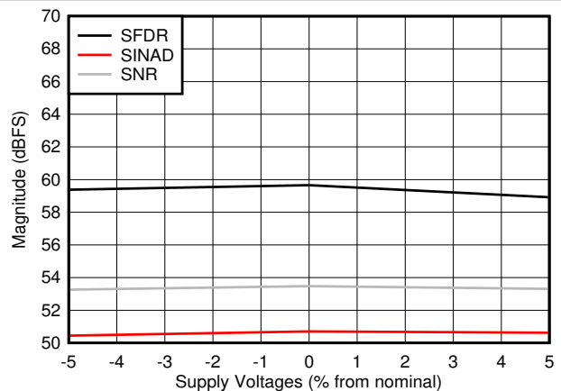
Figure 7-46. SNR, SFDR and SINAD vs Supply Voltage
