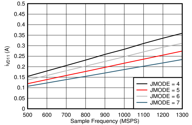
Figure 7-98. Dual Channel, I_{VD11} vs FS and JMODE 4 - 7
