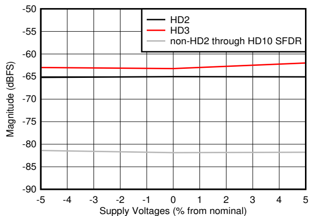
Figure 7-47. HD2, HD3 and Worst non-HD Spur vs Supply Voltage
