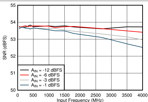
Figure 7-16. SNR vs Input Frequency
