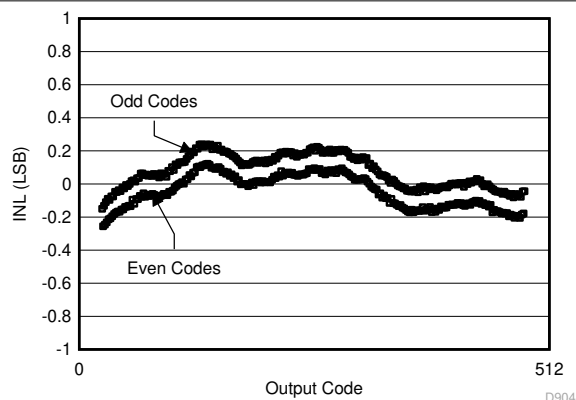
Figure 7-2. INL vs Code
