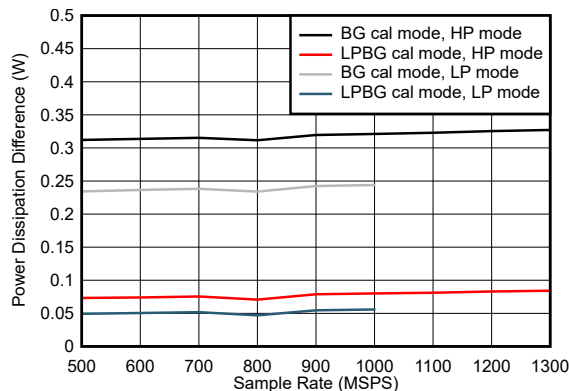
Difference to foreground calibration, JMODE independent Figure 7-113. Single Channel, Power Dissipation Change with Calibration Mode
