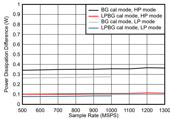
Difference to foreground calibration, JMODE independent Figure 7-111. Quad Channel, Power Dissipation Change with Calibration Mode
