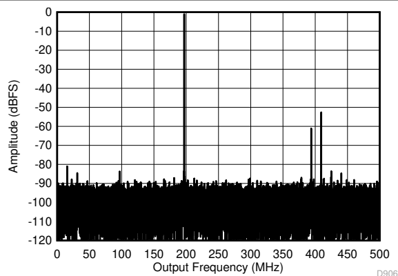
Figure 7-13. Single Tone FFT at 1197 MHz and -1 dBFS
