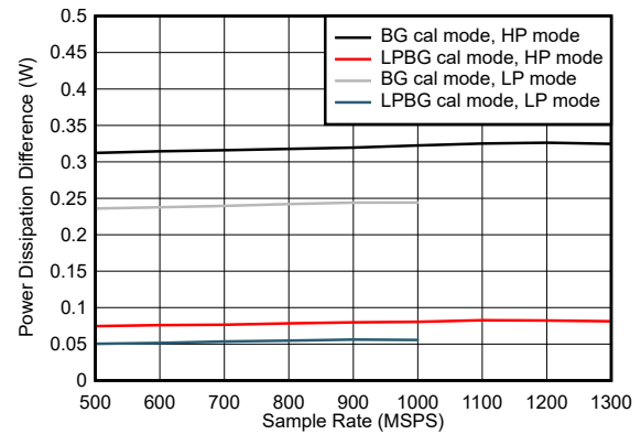
Difference to foreground calibration, JMODE independent Figure 7-112. Dual Channel, Power Dissipation Change with Calibration Mode
