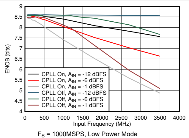
Figure 7-78. ENOB vs Input Frequency, CPLL and Input Amplitude
