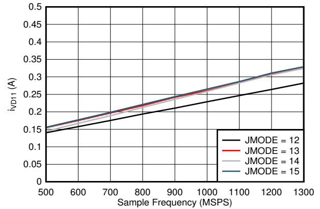
Figure 7-100. Dual Channel, I_{VD11} vs FS and JMODE 12 - 15
