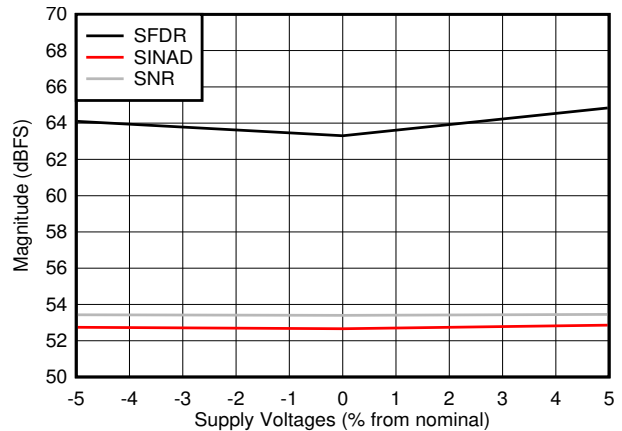
Figure 7-44. SNR, SFDR and SINAD vs Supply Voltage
