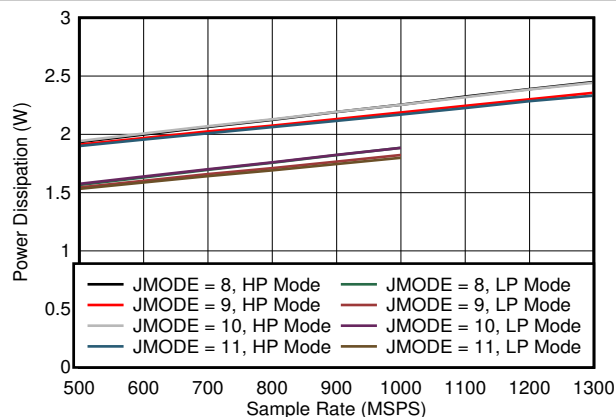
Figure 7-83. Quad Channel, Power Dissipation vs FS for JMODES 8 - 11
