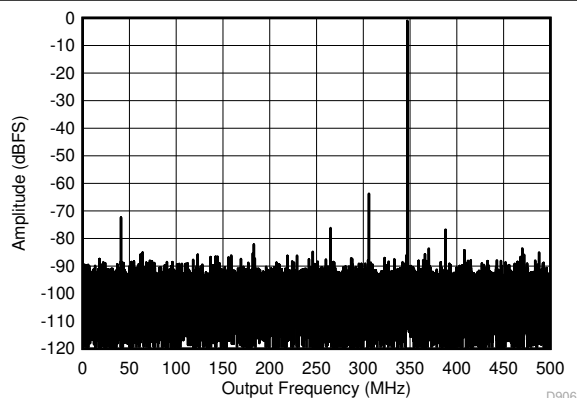
Figure 7-10. Single Tone FFT at 3497 MHz and -1 dBFS
