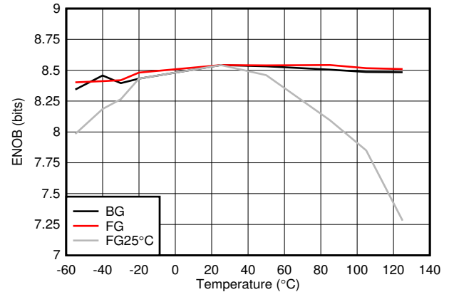
Figure 7-38. ENOB vs Temperature and Calibration Mode
