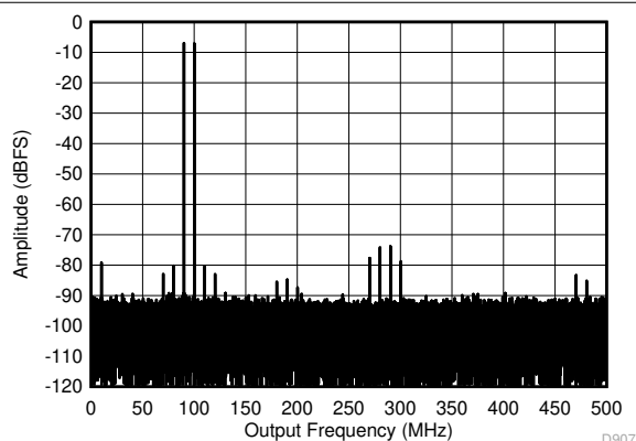
Figure 7-52. Two Tone FFT at 1798 MHz Center
