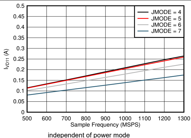
Figure 7-108. Single Channel, I_{VD11} vs FS and JMODE 4 - 7
