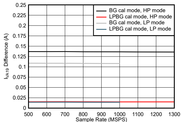
Figure 7-115. Dual Channel, I_{VA19} Change with Calibration Mode
