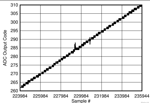
Figure 7-128. Background Calibration Core Transition (AC Signal Zoomed)
