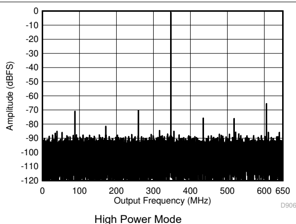
Figure 7-4. Single Tone FFT at 347 MHz and -1 dBFS
