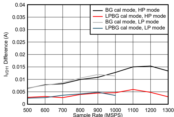
Figure 7-121. Dual Channel, I_{VD11} Change with Calibration Mode
