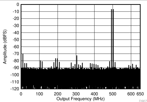
Figure 7-50. Two Tone FFT at 498 MHz Center
