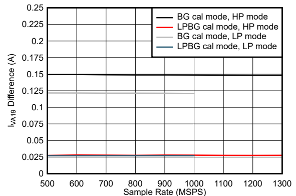
Difference to foreground calibration, JMODE independent Figure 7-114. Quad Channel, I_{VA19} Change with Calibration Mode
