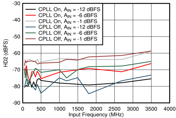
Figure 7-73. HD2 vs Input Frequency, CPLL and Input Amplitude
